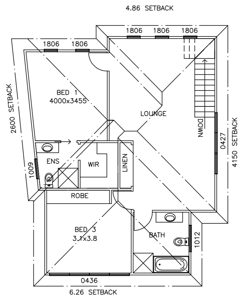
UNIT 2 - FIRST FLOOR
